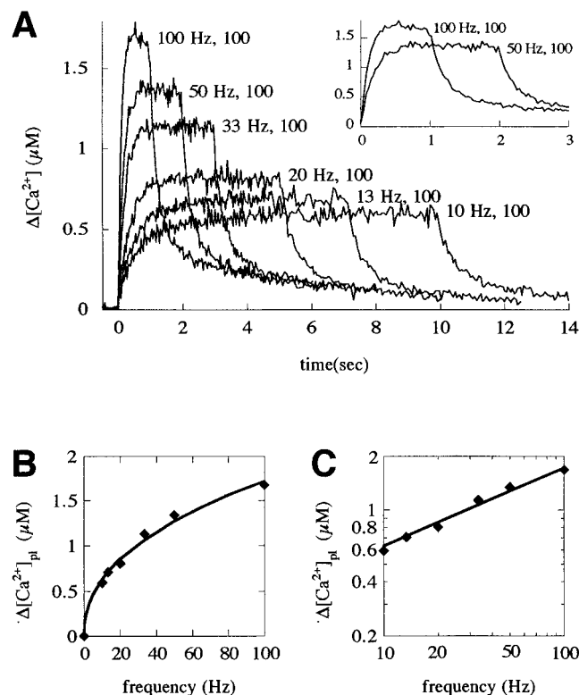
FIGURE 3 Presynaptic changes in [\text{Ca}^{2+}]_i during and after the short-term stimulation at a terminal loaded with OGB-2 (not overloaded). ( A ) Time courses of [\text{Ca}^{2+}]_i changes from the resting level, \Delta[\text{Ca}^{2+}]_i , induced by 100 stimuli with various stimulation frequencies (10–100 Hz). The stimulation started at time zero. Inset shows \Delta[\text{Ca}^{2+}]_i for 50 and 100 Hz stimulation on an expanded time scale. \Delta[\text{Ca}^{2+}]_i reached a plateau after 20–50th stimuli at any stimulation frequency. ( B ) Plateau levels of \Delta[\text{Ca}^{2+}]_i ( \Delta[\text{Ca}^{2+}]_{\text{pl}} ) shown by closed diamonds, obtained by temporally averaging \Delta[\text{Ca}^{2+}]_i during the last 20 (80th to 100th) stimuli, plotted against the stimulation frequency. ( C ) A log-log plot of B . The data points were best fitted using Eq. 9, with n = 2.16 ( 2.01 \pm 0.10 , mean \pm SE, N = 8 ) and \delta_{\text{CaT}}/\gamma = 0.036 ( 0.031 \pm 0.006 , mean \pm SE, N = 8 ). Estimated concentration of OGB-2 was about 200 \mu\text{M} in this terminal.
